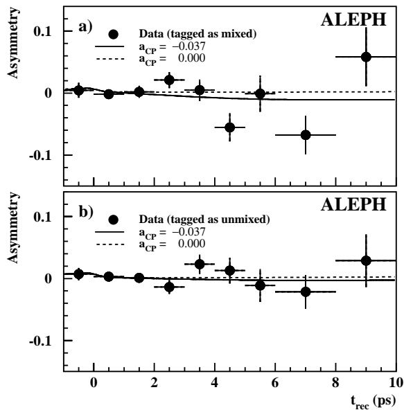
Fig. 1. a Final state asymmetry in events tagged as mixed. b Final state asymmetry in events tagged as unmixed. In each plot, the expectation for a_{CP} = 0 (dashed line) and the result of the fit for a_{CP} (solid line) have been superimposed. The positive asymmetry at zero proper time is due to fake leptons
