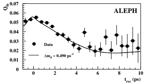
Fig. 3. Average lepton-signed hemisphere charge Q_{\ell h} as a function of proper time, with the fit result superimposed
