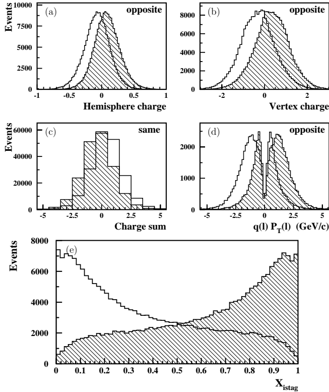
Fig. 4a–e. Distributions of the discriminating variables a–d and of the combined discriminant e used for initial-state tagging. The open (hatched) histograms are for hemispheres in which a B^0 ( \bar{B}^0 ) was produced in Monte Carlo
