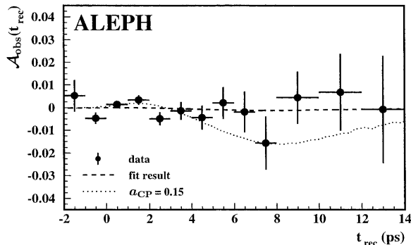
Fig. 5. Observed time-dependent asymmetry \mathcal{A}_{\text{obs}}(t_{\text{rec}}) between tagged \bar{b} and b hemispheres, with the result of the fit superimposed (dashed line). Also shown for illustration is the predicted curve for a_{\text{CP}} = 0.15 (dotted line)
