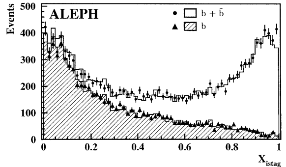
Fig. 6. Distribution of the initial state tagging variable X_{\text{istag}} for b and \bar{b} enriched hemispheres in data (points) and Monte Carlo (histograms)
