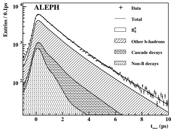
Fig. 2. Proper time distribution of the selected events and result of the lifetime fit
